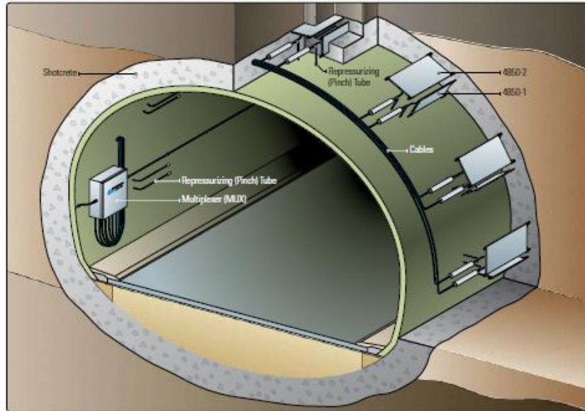
● Illustration shows typical installation in tunnel lining.
